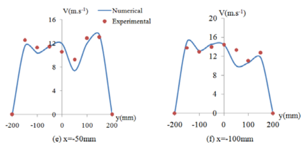
Fig. 14 Velocity profile in the plane z=50 mm
