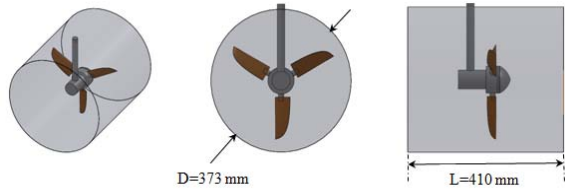
Fig. 2 Rotating area
