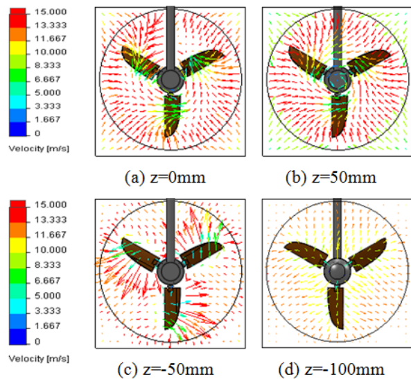
Fig. 6 Velocity fields in the transverse planes
