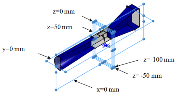
Fig. 4 Compliance planes
