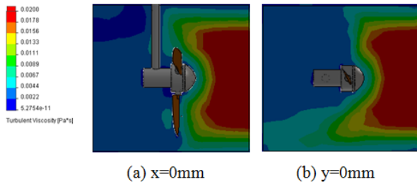
Fig. 12 Turbulent viscosity in the longitudinal planes
