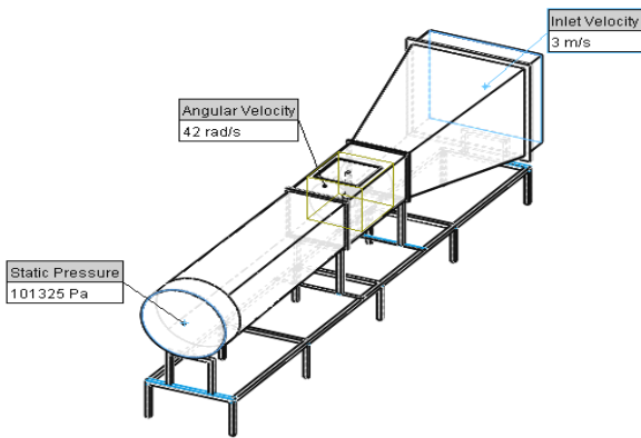
Fig. 3 Boundary conditions
