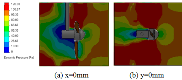
Fig. 9 Dynamic pressure in the longitudinal planes
