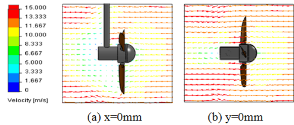
Fig. 5 Velocity fields in the longitudinal planes
