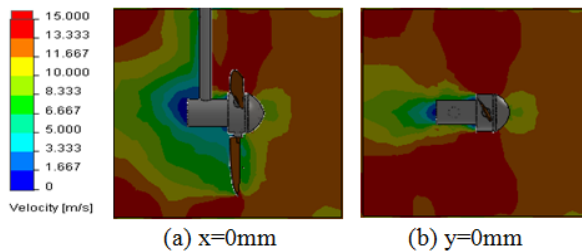
Fig. 7 Average velocity in the longitudinal planes
