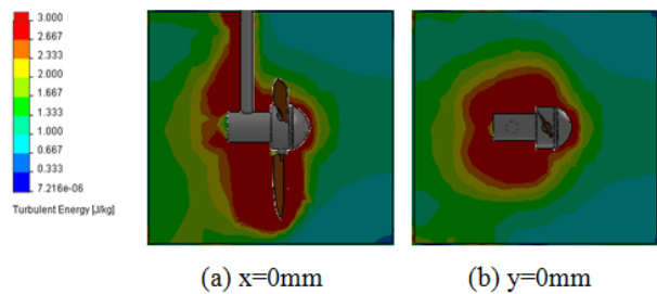
Fig. 10 Turbulent kinetic energy in the longitudinal planes
