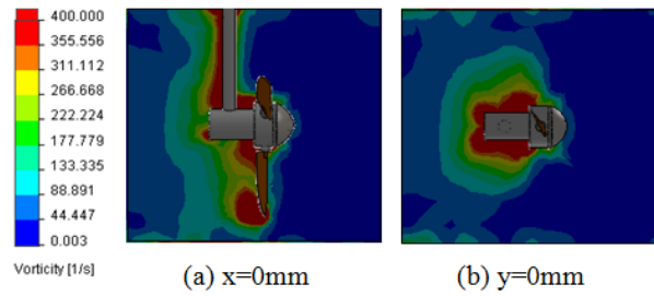
Fig. 13 Vorticity in the longitudinal planes
